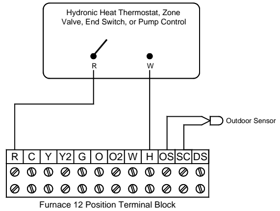
Model 7140 - Single Hydronic Heating Zone Application
